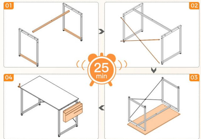
Figure 2: Quick and easy assembly process for the ODK desk.
