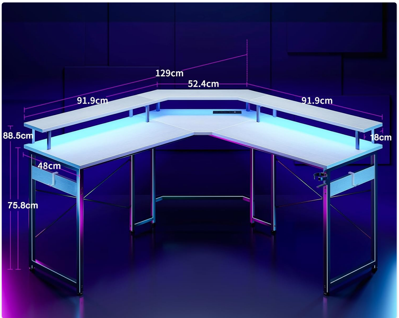
Image 6.1: Detailed dimensions of the ODK Gaming Corner Desk.
