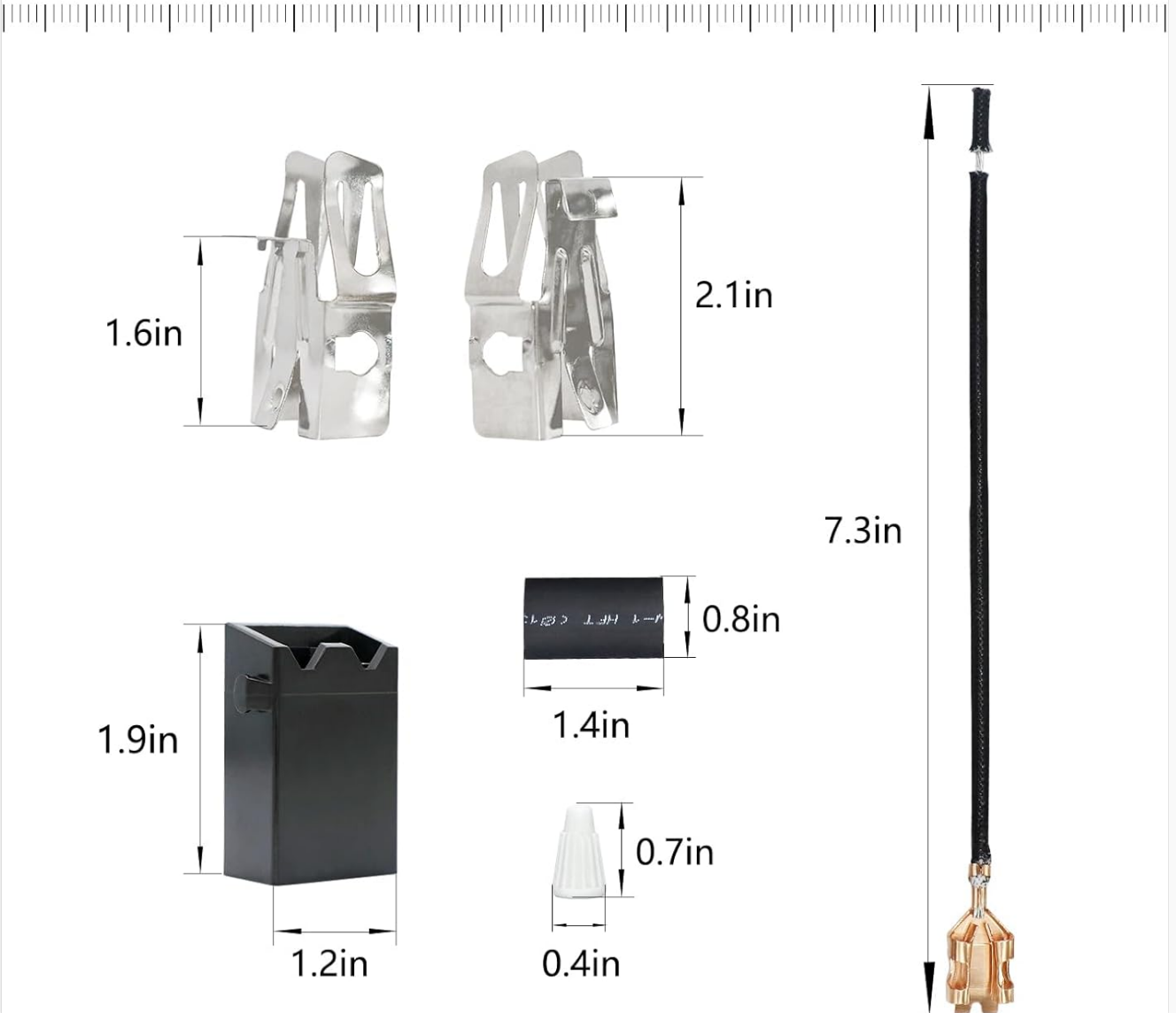
Image 6.1: Detailed dimensions of the kit components.
