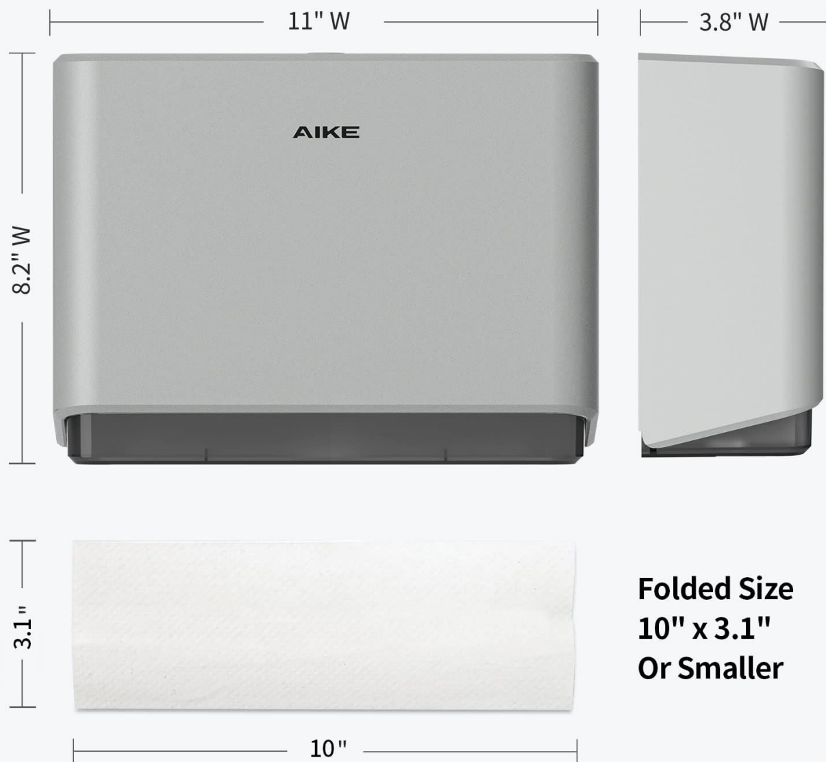
Image: The AIKE Paper Towel Dispenser (AK5101) with its key dimensions labeled, including width, height, and depth, and compatible paper towel size.
