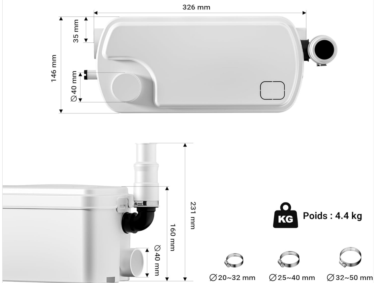
Figure 8.2: Product dimensions.
