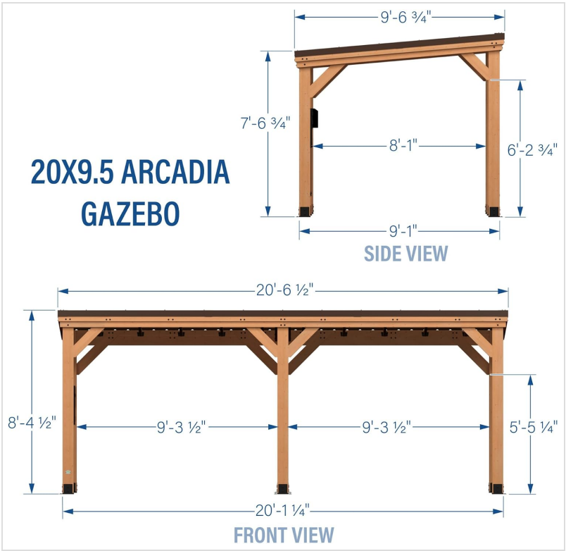
Detailed dimensions for the 20x9.5 Arcadia Gazebo, showing side and front views with key measurements.
