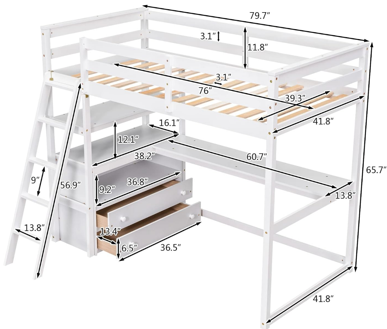
Figure 7.1: Dimensional diagram of the Merax Twin Loft Bed, showing all key measurements in inches.
