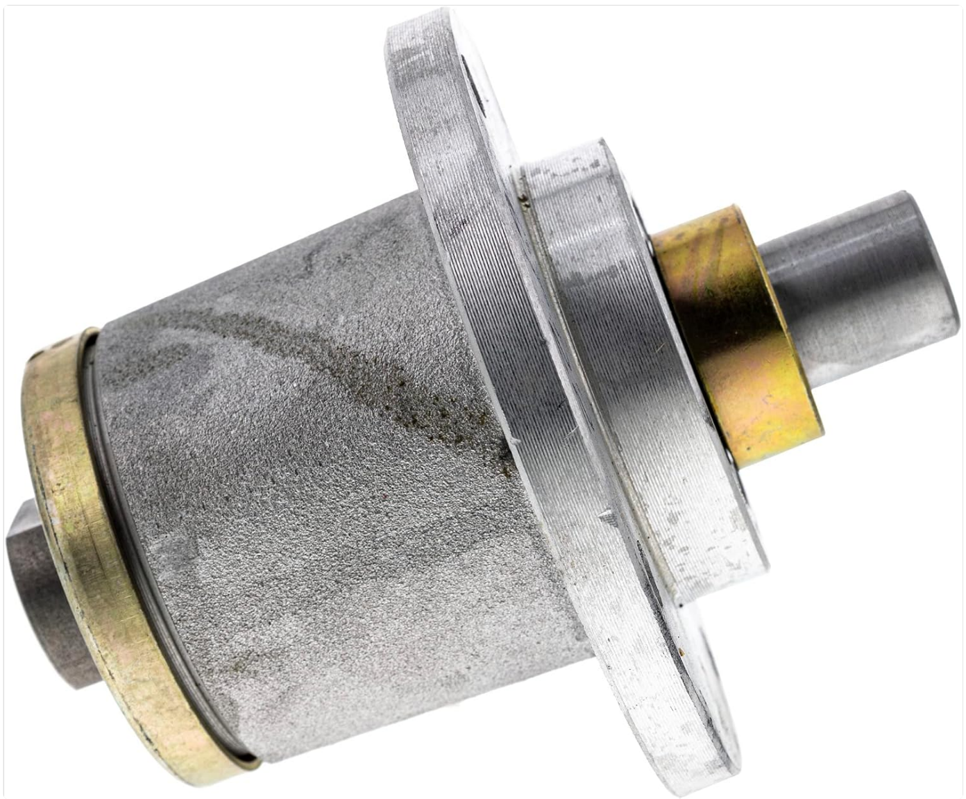
Side view of the Spartan Mowers 437-0006-00 Deck Spindle, showing its cylindrical body and mounting flange.
