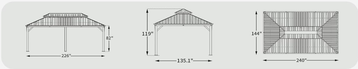
Figure 3: Detailed product dimensions to assist with planning and assembly.
