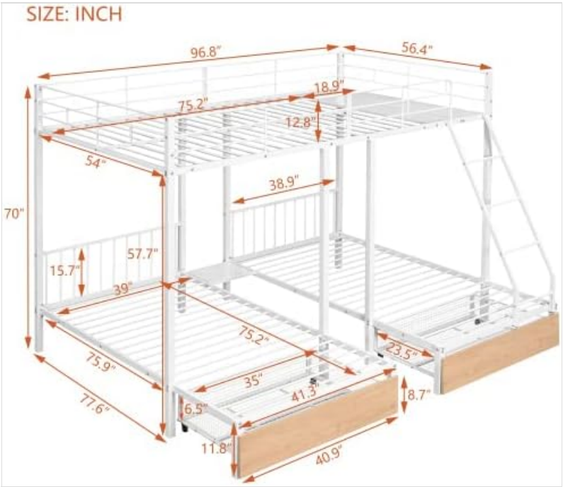
Image: Detailed dimensions diagram for the Bellemave Full Over Twin Triple Bunk Bed, showing length, width, and height measurements for all sections.
