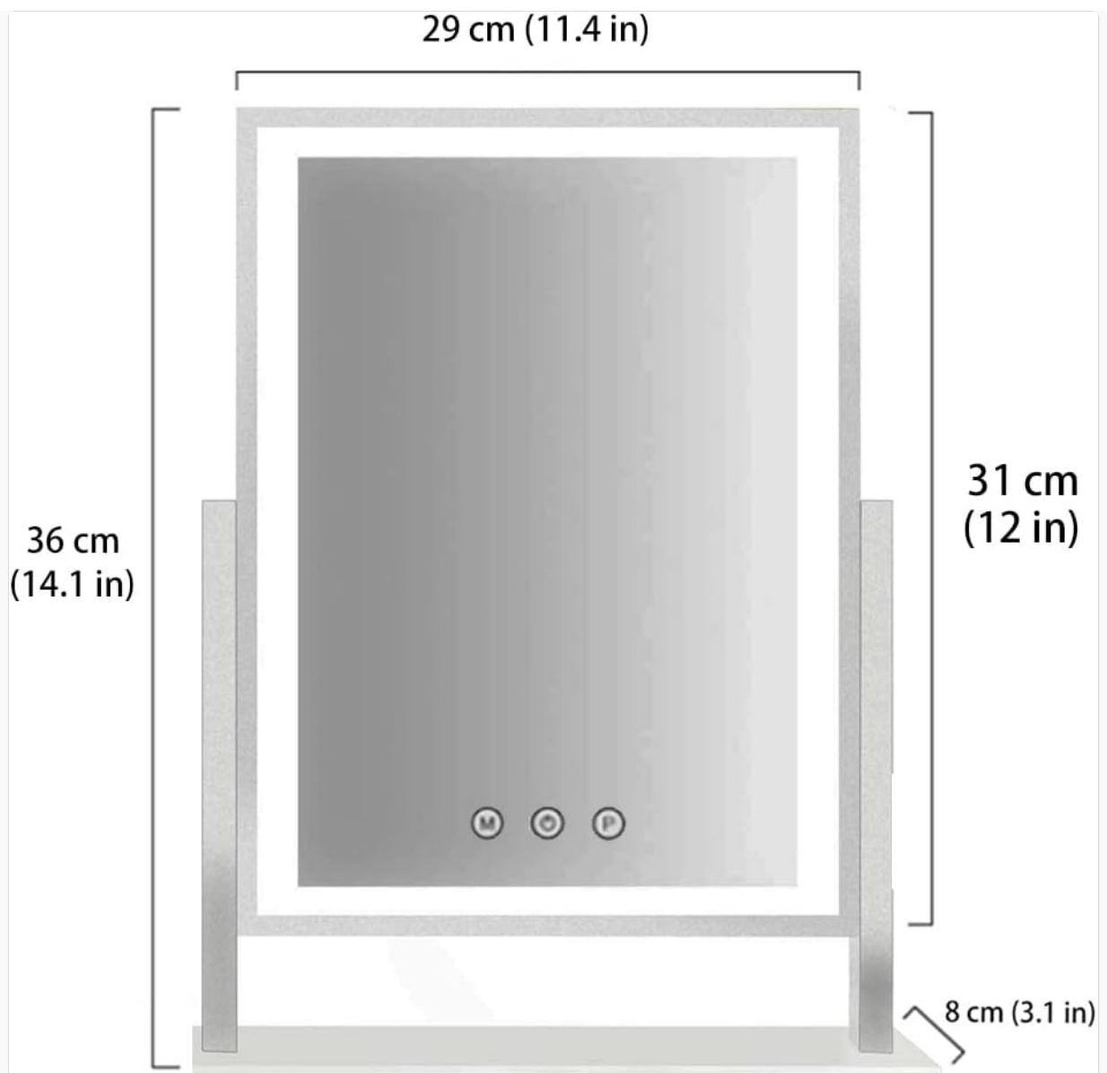
Image: Dimensional diagram of the mirror, illustrating its physical measurements.
