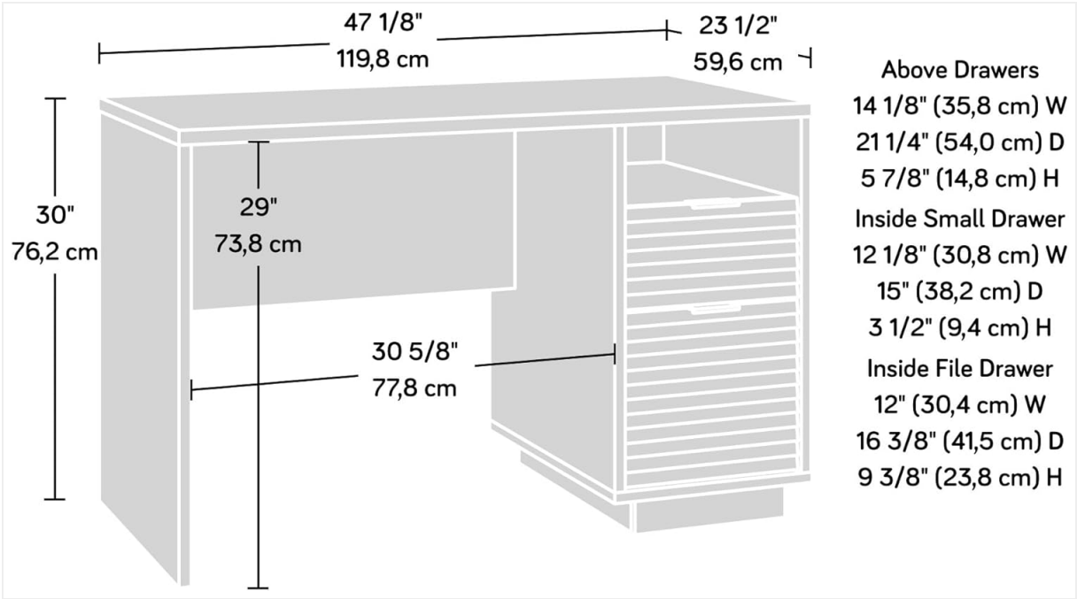
Image: Dimensional diagram of the desk, including measurements for overall size and internal drawer/shelf spaces.
