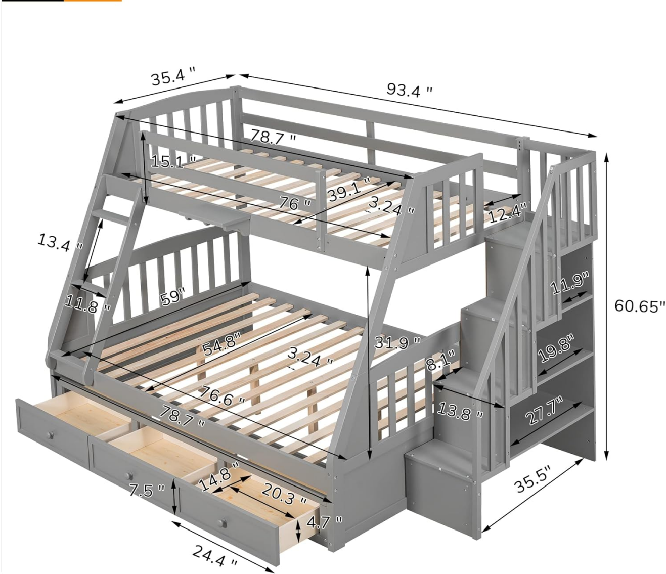
Image: A technical diagram illustrating the detailed dimensions of the Bellemave Twin Over Full Bunk Bed, including length, width, height, and internal measurements for both bunks and storage components.
