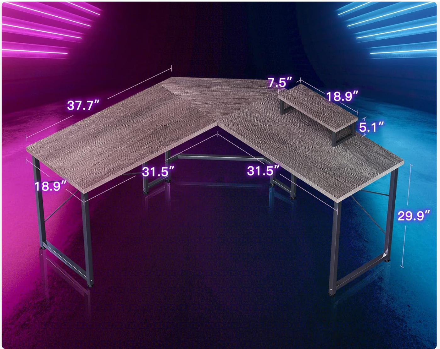
Image 2.1: A diagram illustrating the dimensions of the ODK L Shaped Gaming Desk, including the main desktop sections and the monitor stand. Key measurements are shown in inches.
