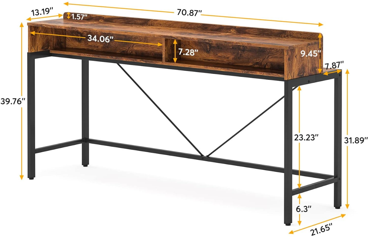
Image: Detailed dimensions of the sofa console table for accurate placement and planning.
