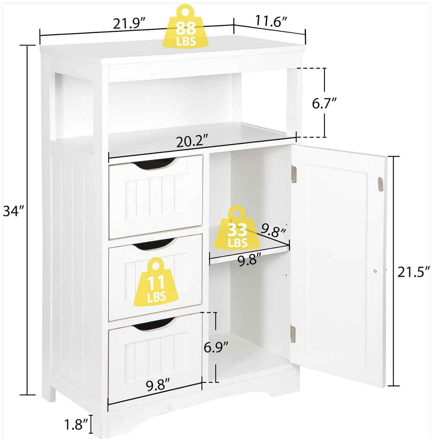
Figure 6: Detailed dimensions and weight capacities for the ZenStyle Bathroom Floor Cabinet.
