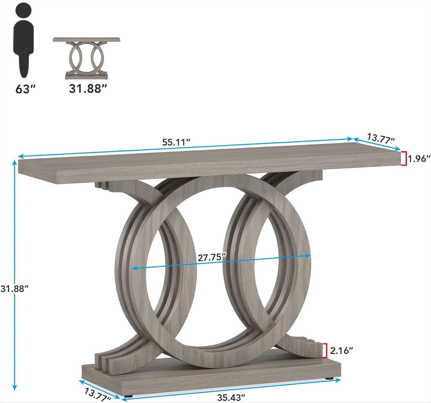
Figure 4.1: Product dimensions for assembly planning.
