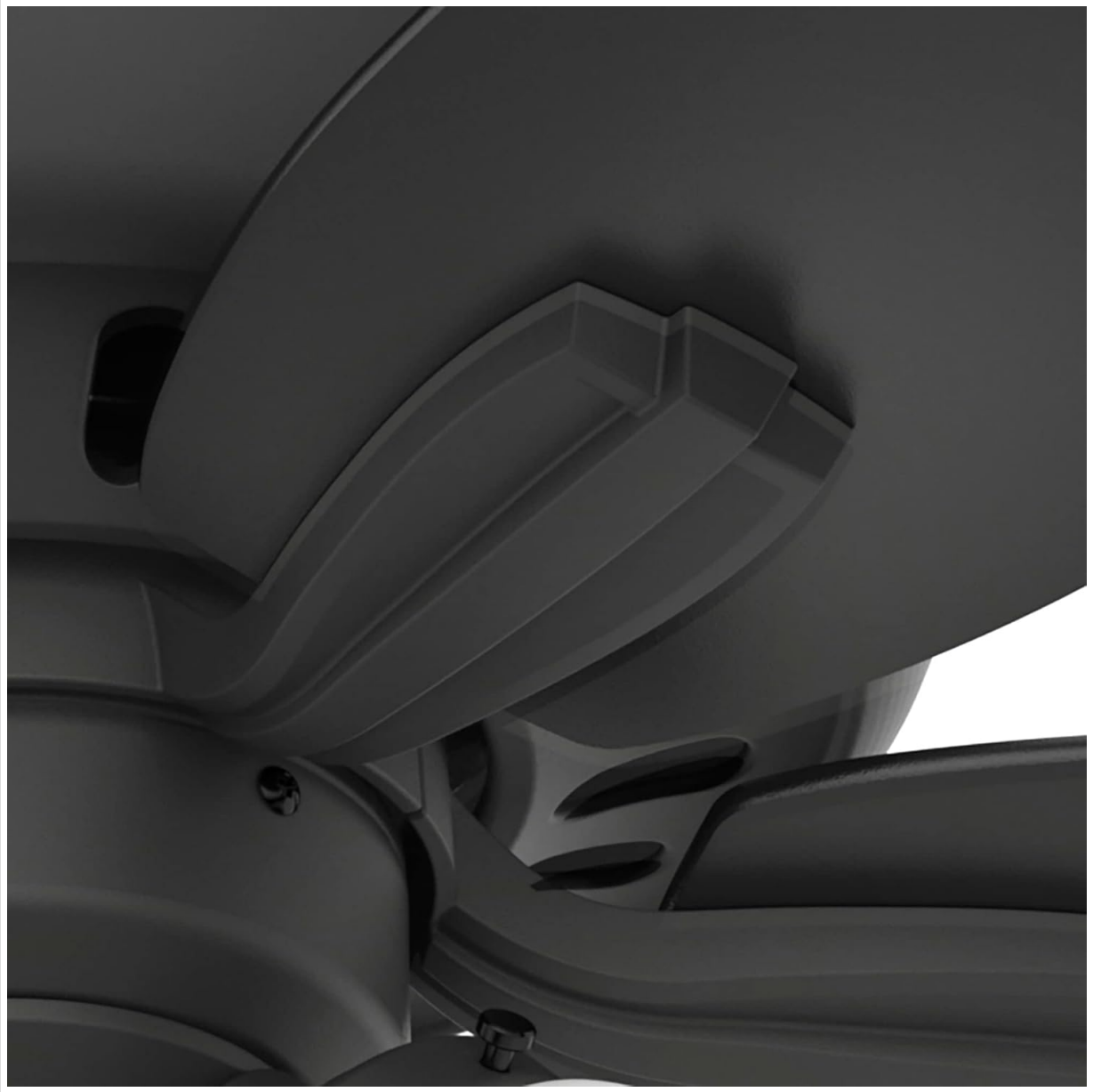
Image 5.2: Blade Attachment Detail. This close-up view illustrates the method for securing a fan blade to the motor housing using screws, highlighting the connection point.
