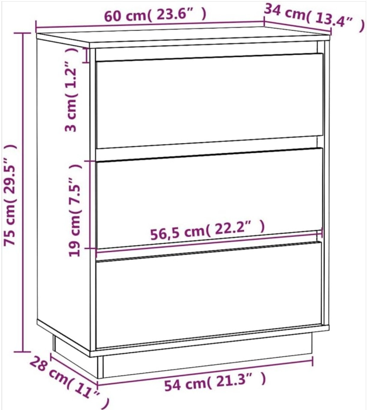
Figure 1: Product Dimensions. Refer to this diagram for overall measurements during assembly and placement.
