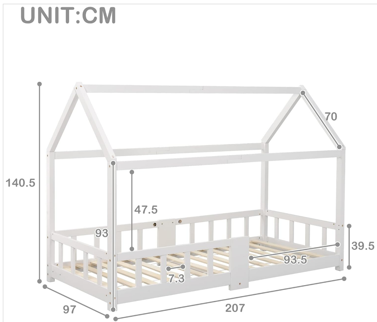
Figure 1: Dimension diagram of the SEGMART Children's Wooden House Bed. This diagram illustrates the overall dimensions of the bed frame, including length (207 cm), width (97 cm), and height (140.5 cm). Key measurements for the bed base and roof structure are also provided.
