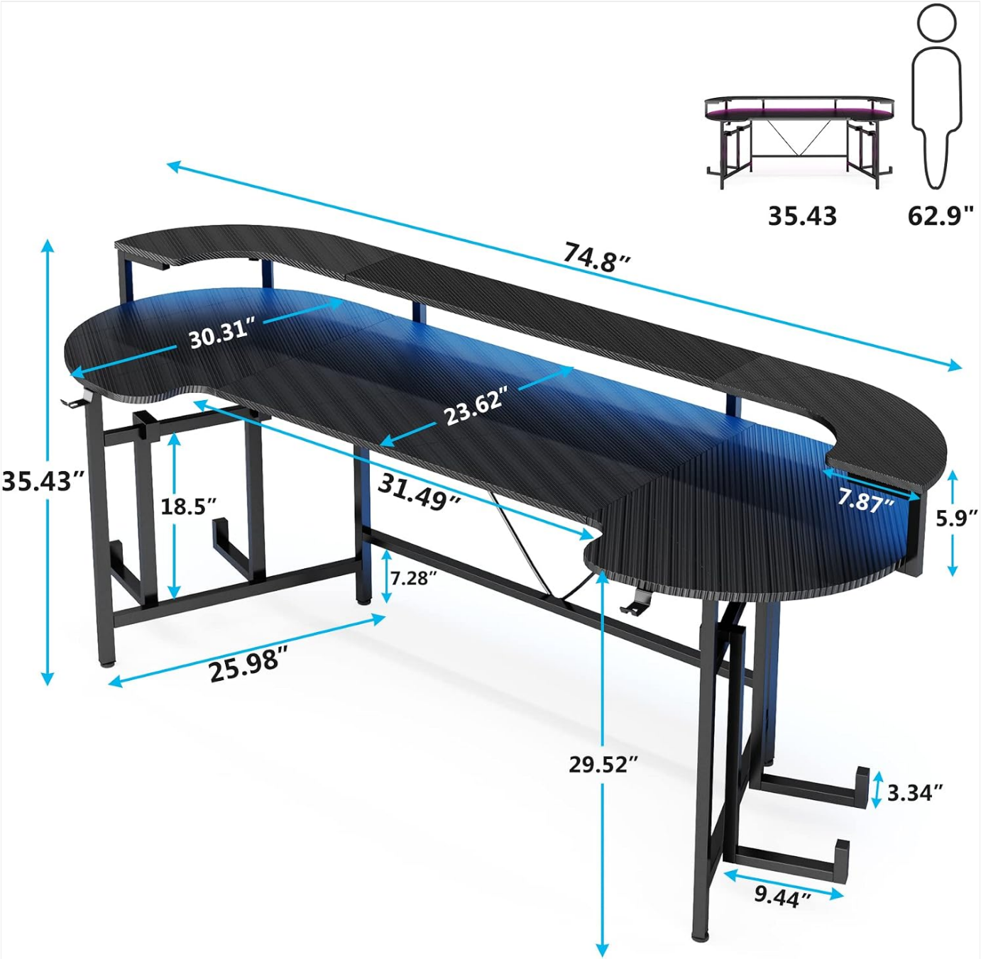
Image: A detailed diagram illustrating the dimensions of the Tribesigns 75-inch Gaming Desk, including height, width, and depth measurements for various sections.
