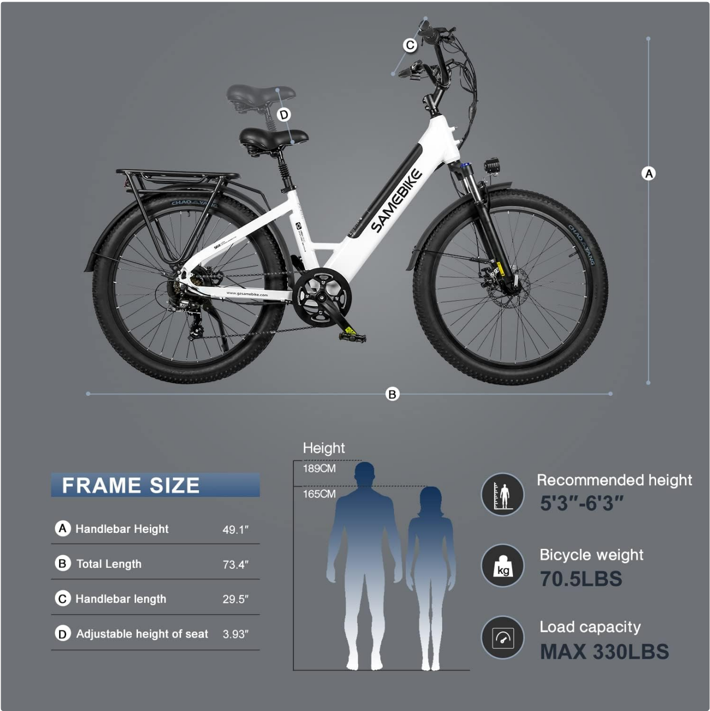
Figure 2: Frame size and recommended rider height for the SAMEBIKE RS-A01. This diagram illustrates key dimensions such as
