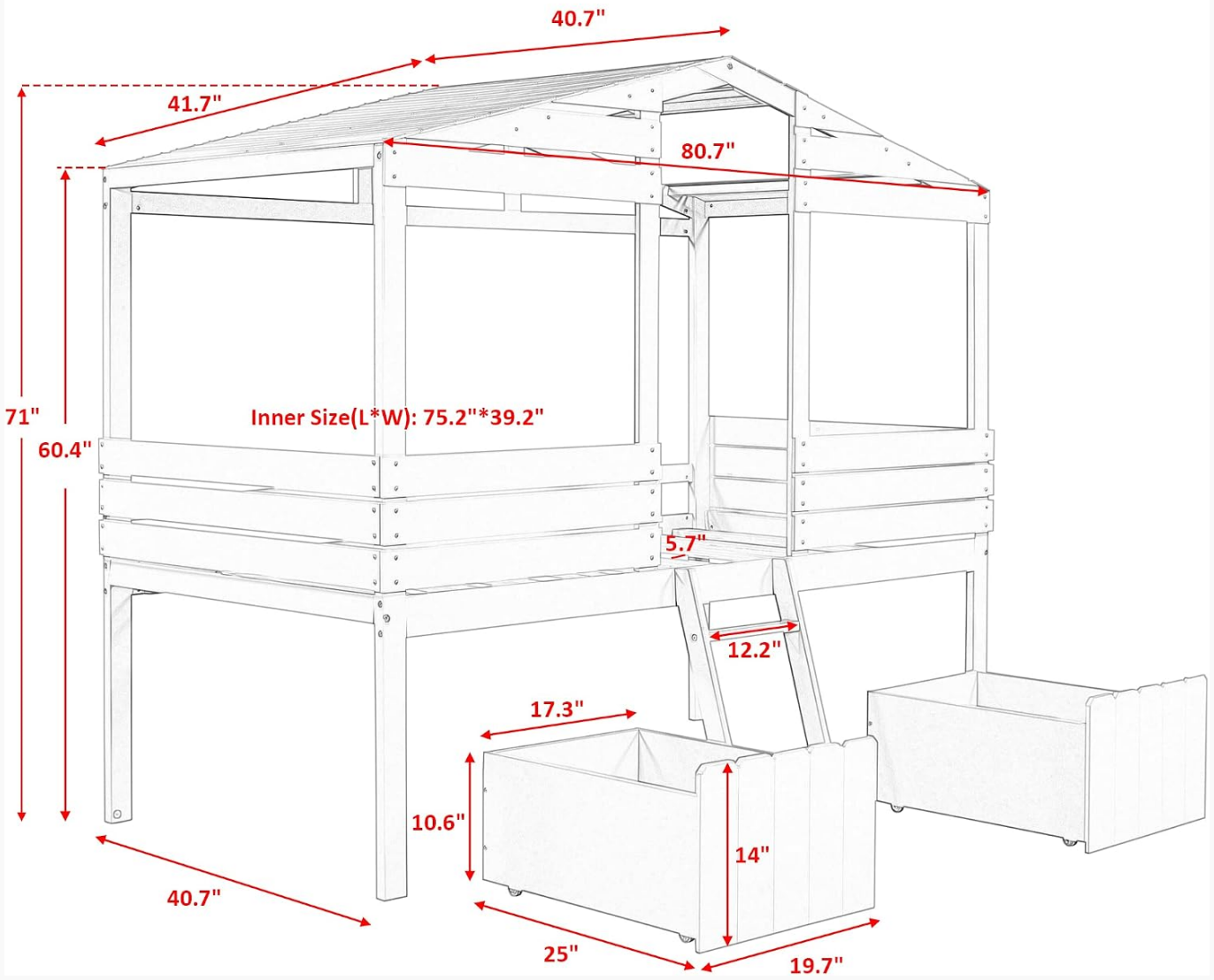
Figure 8.1: Product Dimensions Diagram.
