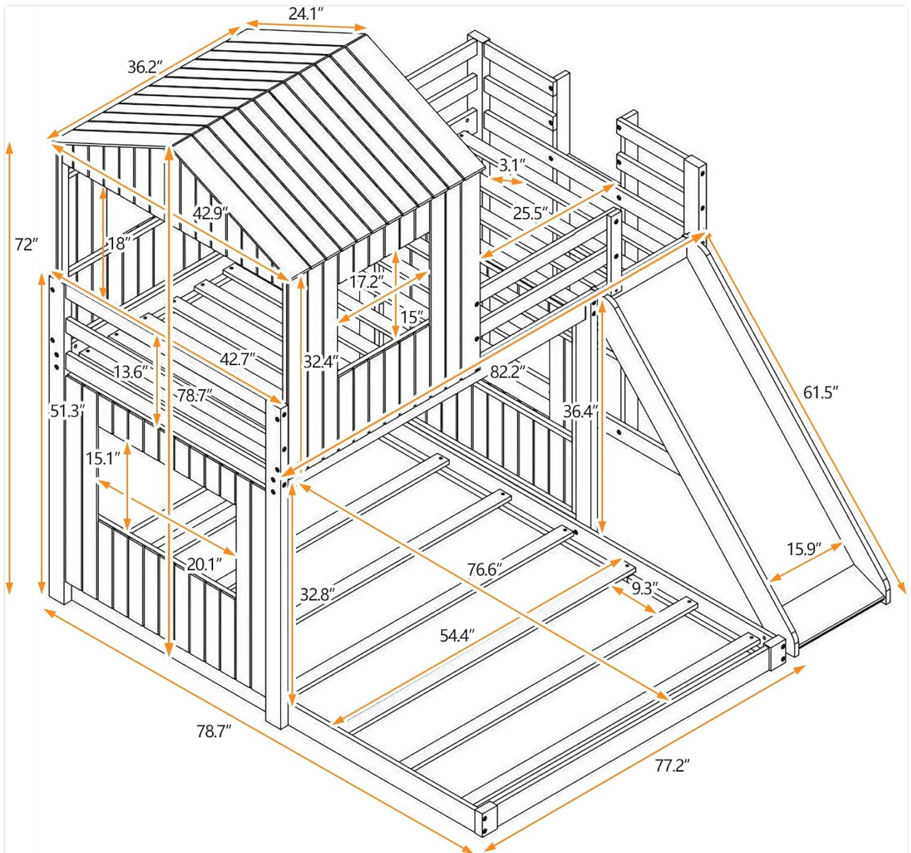
Figure 2.1: Detailed dimensions diagram for the KLMM Twin Over Full Bunk Bed. This illustration provides precise measurements for all components, aiding in assembly and space planning.
