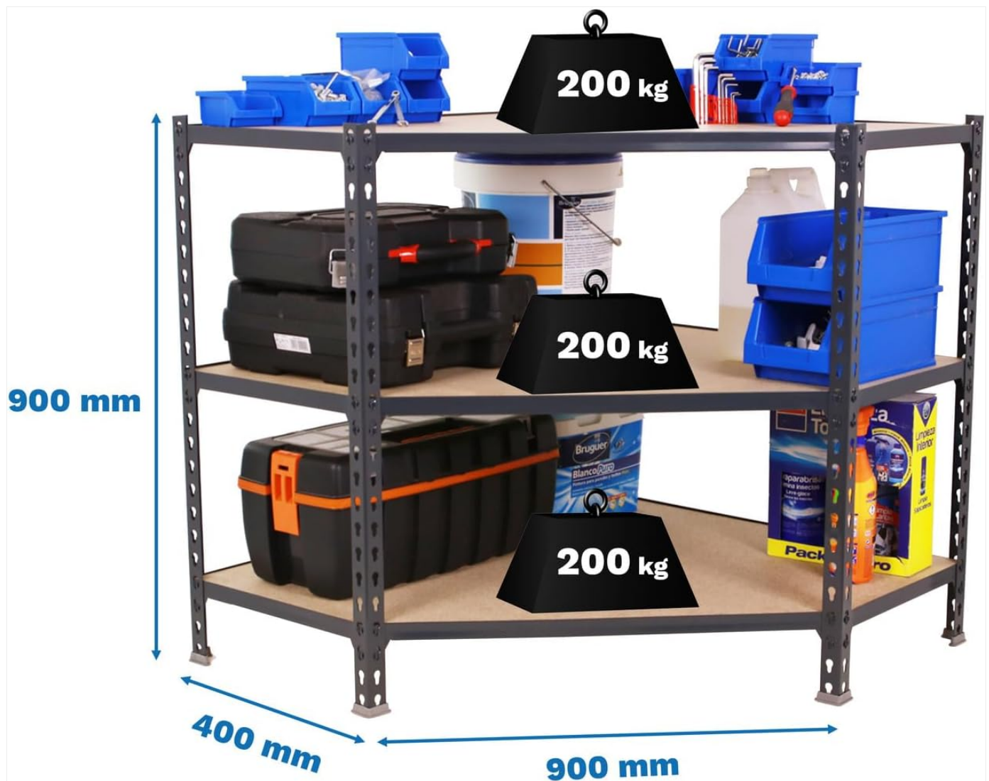
Image: The corner shelf displaying its dimensions (900mm H x 900mm W x 400mm D) and indicating a 200 kg load capacity per shelf.
