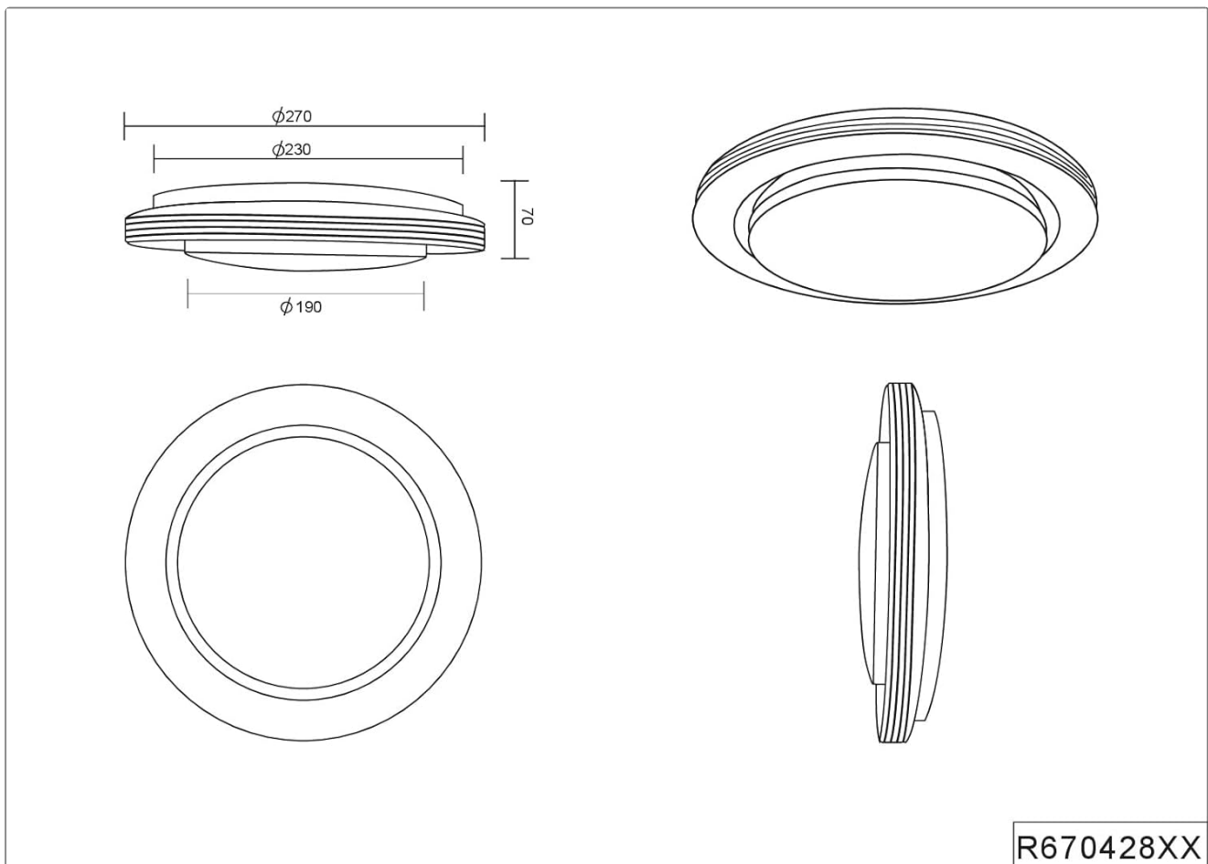
Image 4.1: Technical drawing showing dimensions (Diameter 270mm, Height 70mm) for installation planning.
