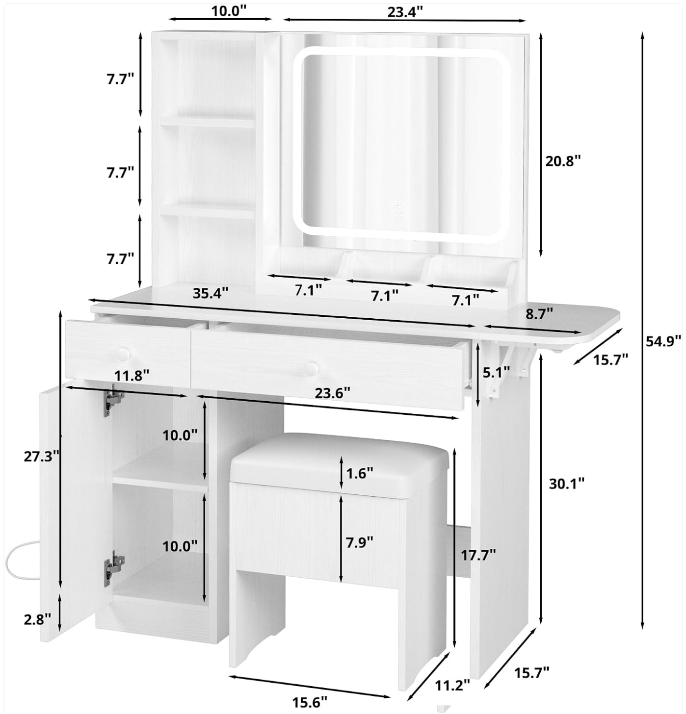
Figure 2: Product dimensions for planning placement.
