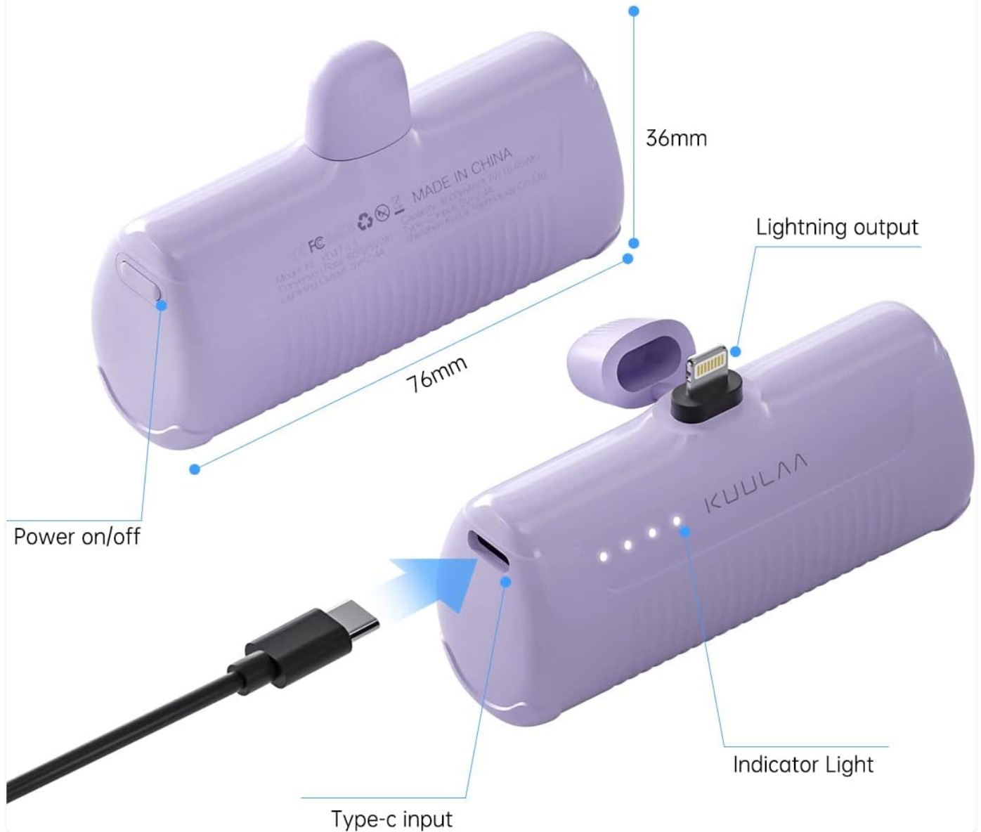
Figure 2: Diagram illustrating the Type-C input port and the four LED indicator lights on the power bank.
