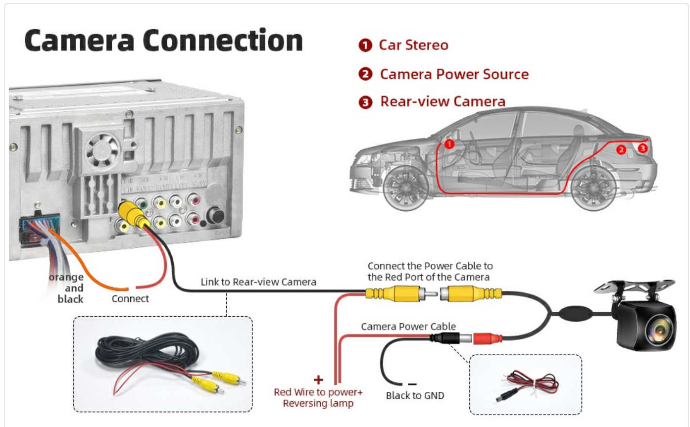
Image: A diagram illustrating how to connect the rear view camera to the car stereo. It shows the camera, video cable, and power connections to the car's reversing lamp and ground.
