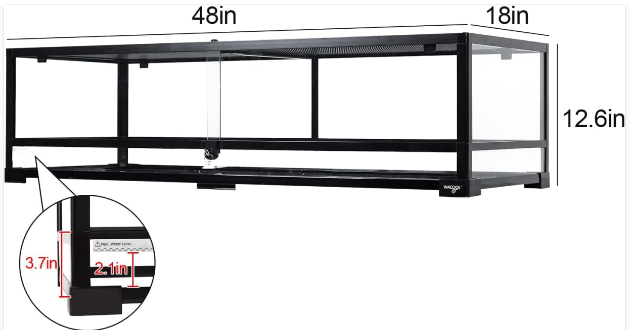
Image 7.1: Dimensional drawing of the WACOOOL TERRA 45 Gallon Reptile Terrarium.
