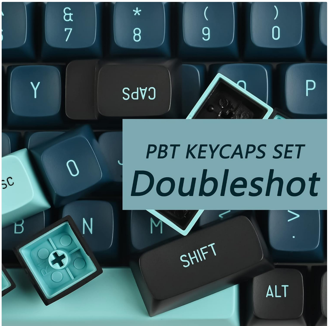
Figure 2.2: A close-up view illustrating the PBT Doubleshot construction, where two layers of plastic are molded together for durable legends.
