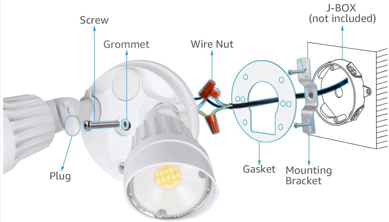
Image: Exploded view of the security light showing the fixture, mounting bracket, gasket, wire nuts, and screws.
