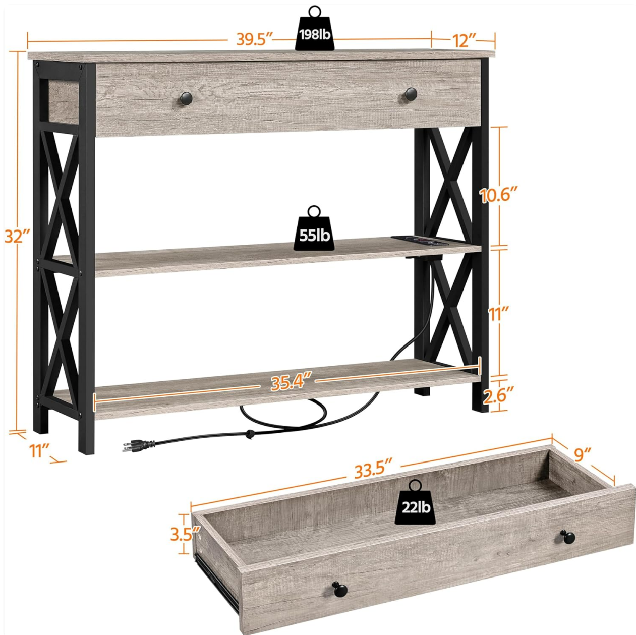
Image: Diagram showing the console table's dimensions: 39.5" L x 12" W x 32" H. Top shelf capacity: 198 lbs, middle/bottom shelf capacity: 55 lbs, drawer capacity: 22 lbs.
