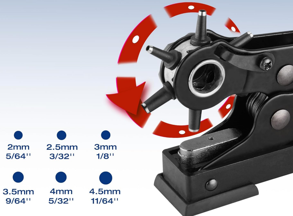
Figure 2: Detail of the rotary punch head, illustrating the six available hole sizes for diverse applications.
