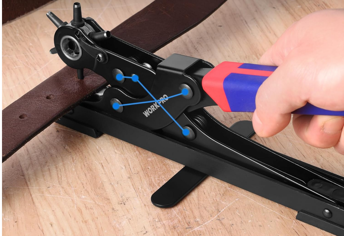
Figure 5: Demonstrating the lever mechanism for punching a hole in a leather belt.
