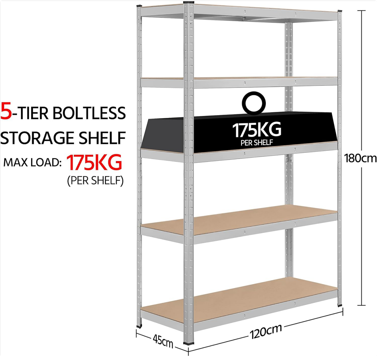
Figure 2: Product Dimensions and Load Capacity
