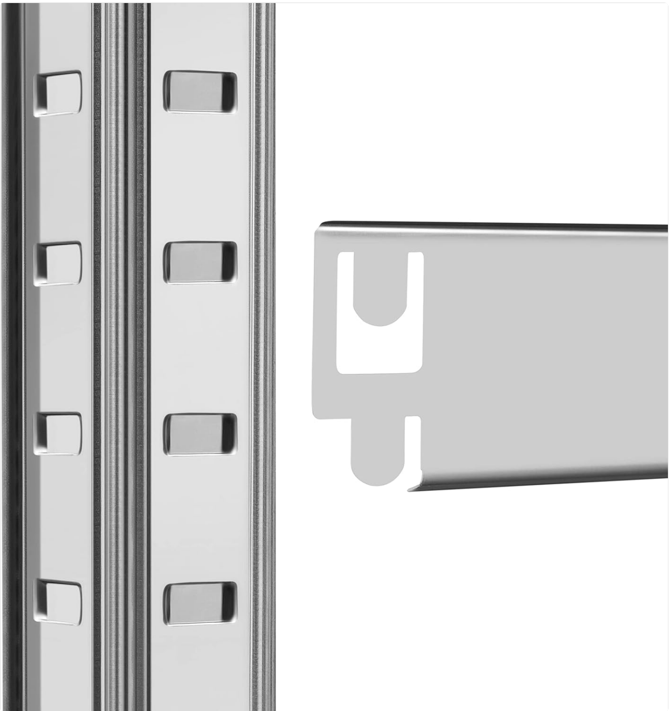
Figure 7: Boltless Connection
