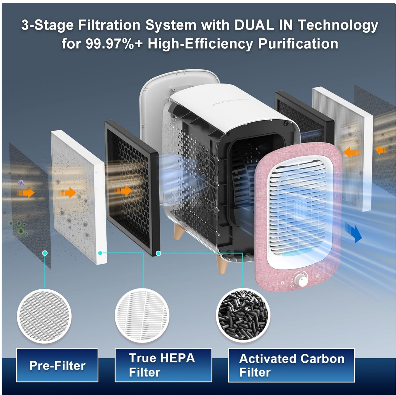
Image: An exploded view diagram illustrating the three layers of the filtration system: Pre-Filter, True HEPA Filter, and Activated Carbon Filter.
