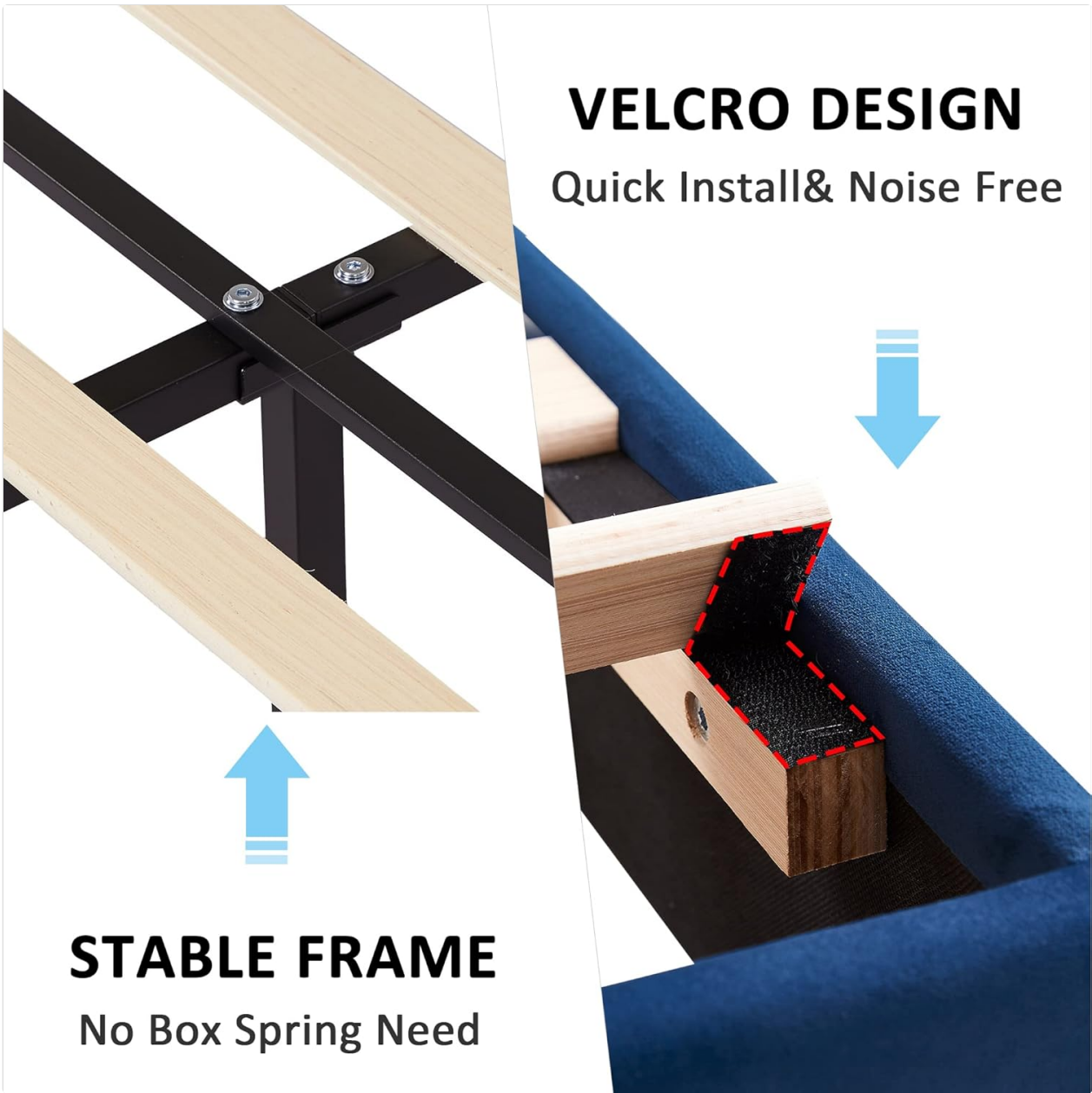
Image 4.3: Detail of the Velcro design, highlighting how wooden slats are quickly and securely attached to the bed frame for stability and noise reduction.
