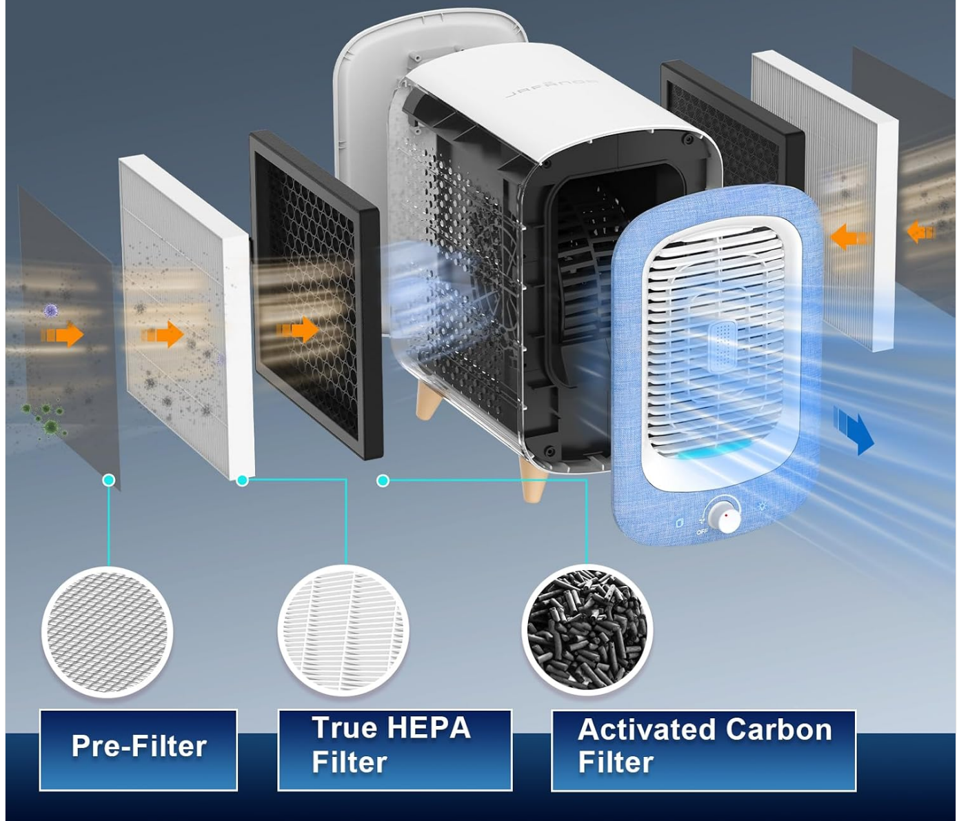
Image: Exploded view illustrating the three-stage filtration system, including the pre-filter, True HEPA filter, and activated carbon filter, and their placement within the unit.
