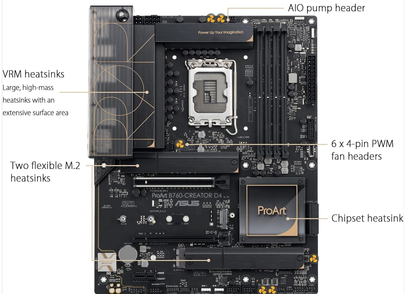
Image Description: An overhead view of the motherboard highlighting its comprehensive cooling features. Labels point to the large, high-mass VRM heatsinks with extensive surface area, two flexible M.2 heatsinks, six 4-pin PWM fan headers, an AIO pump header, and the chipset heatsink, all designed to dissipate heat effectively.
