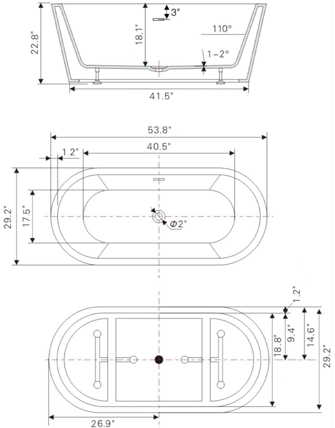
Image: Detailed dimensions and structural diagram of the bathtub.
