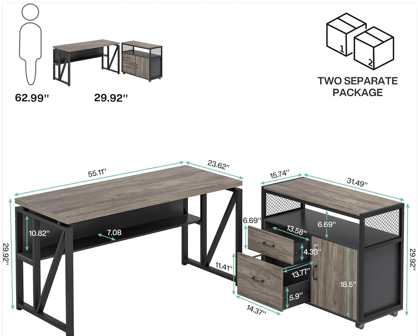
Assembly diagram showing the desk and cabinet with key dimensions for proper setup.
