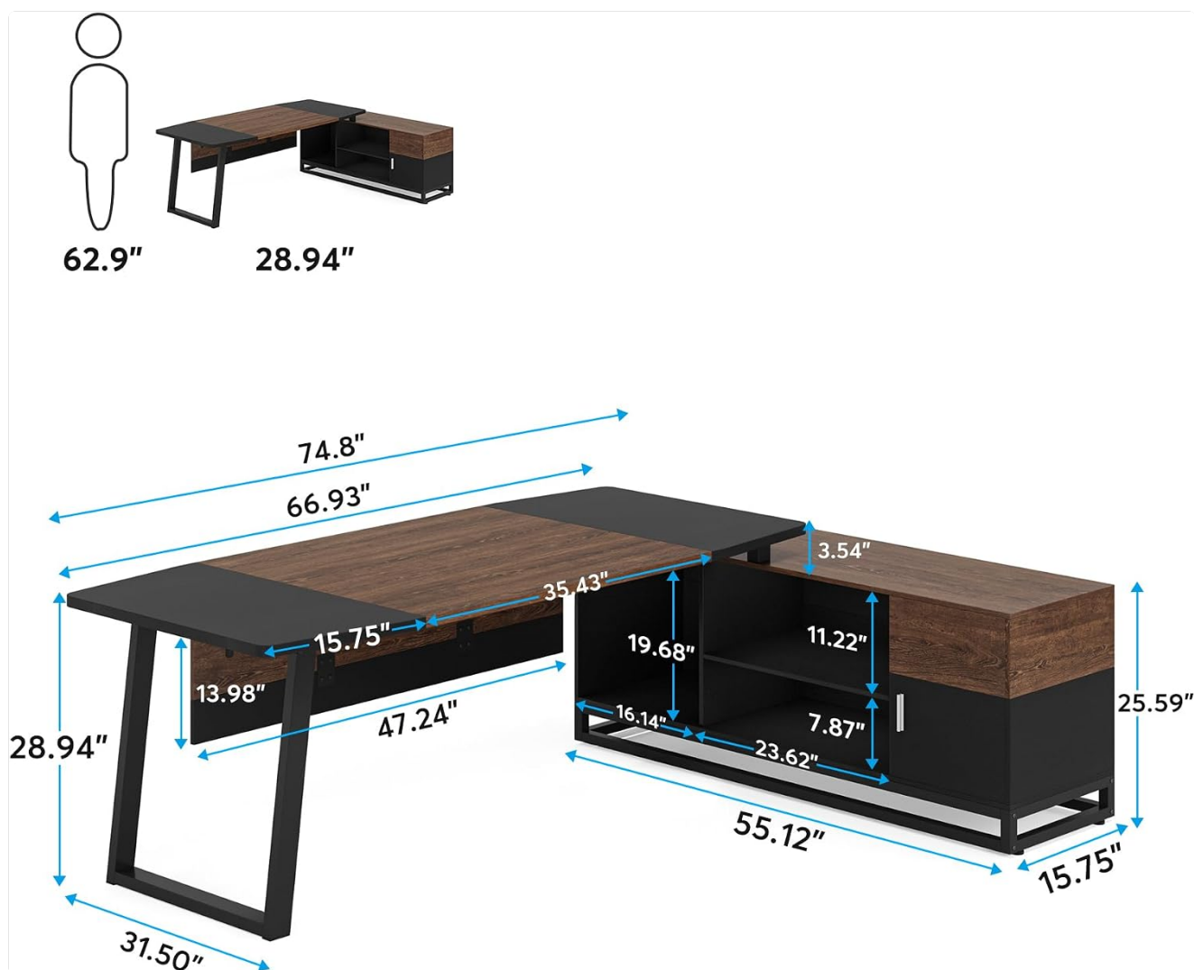
Figure 3.1: Product Dimensions for planning your space.
