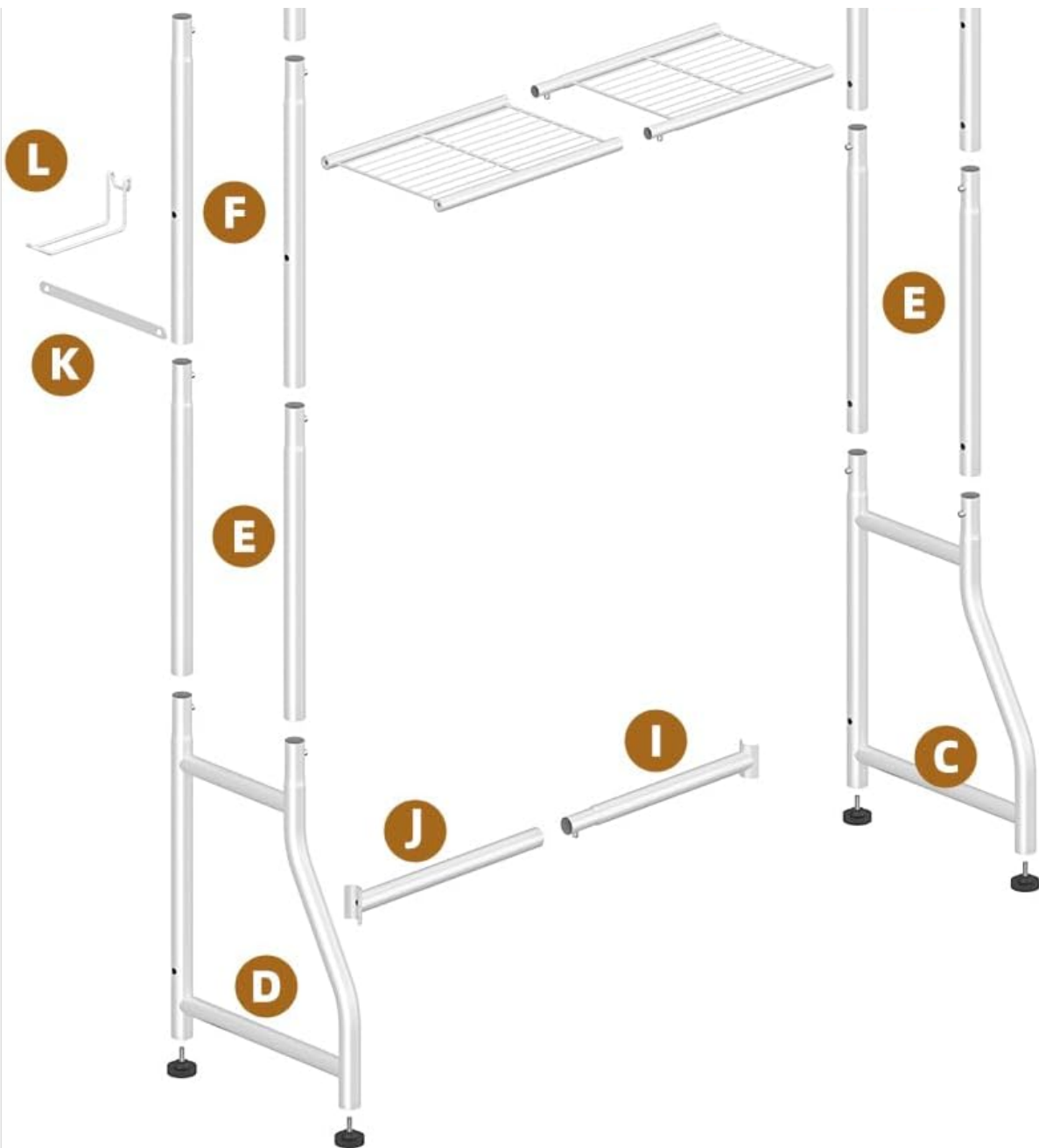
Figure 1: Assembly Diagram with labeled parts (A-L).
