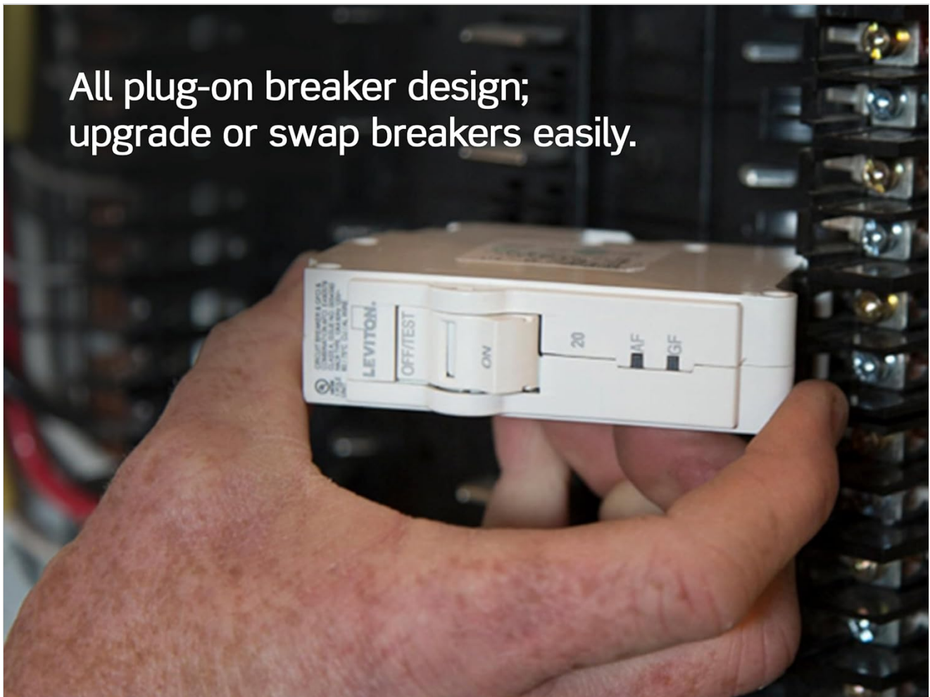
Figure 4.1: A hand demonstrating the installation of a plug-on circuit breaker into the load center bussing.
