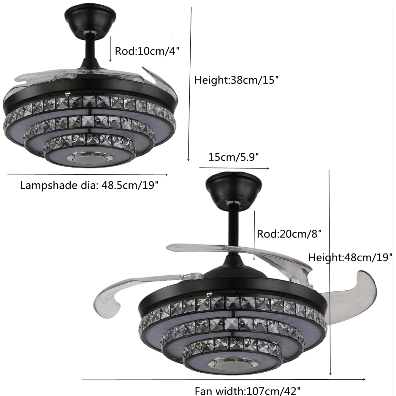
Image 4.1: Fan dimensions with both 4-inch (10cm) and 8-inch (20cm) downrod options. Fan width is 42 inches (107cm) when blades are expanded, and lampshade diameter is 19 inches (48.5cm).
