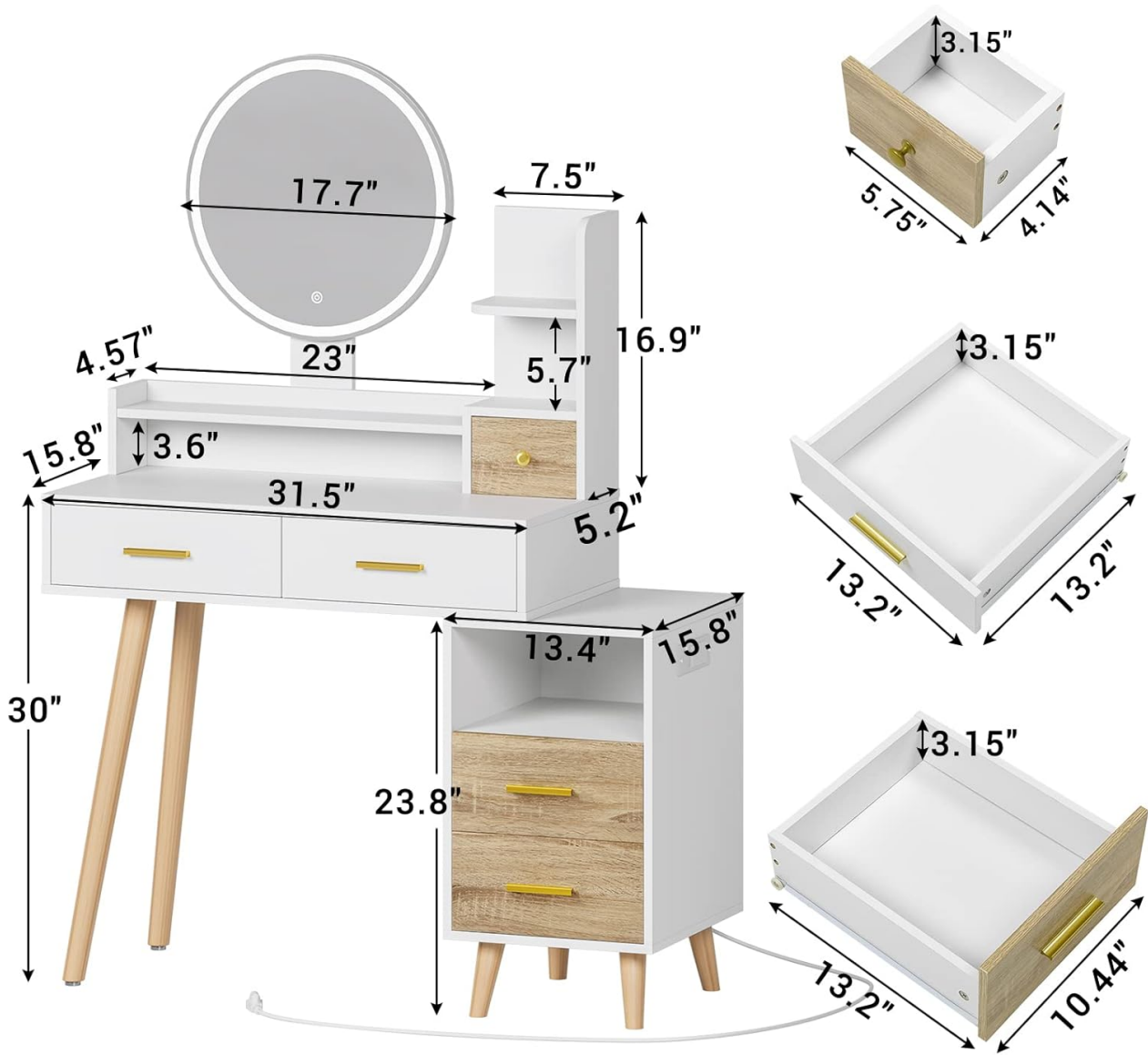
Image 4.1: Product Dimensions and Exploded View.
