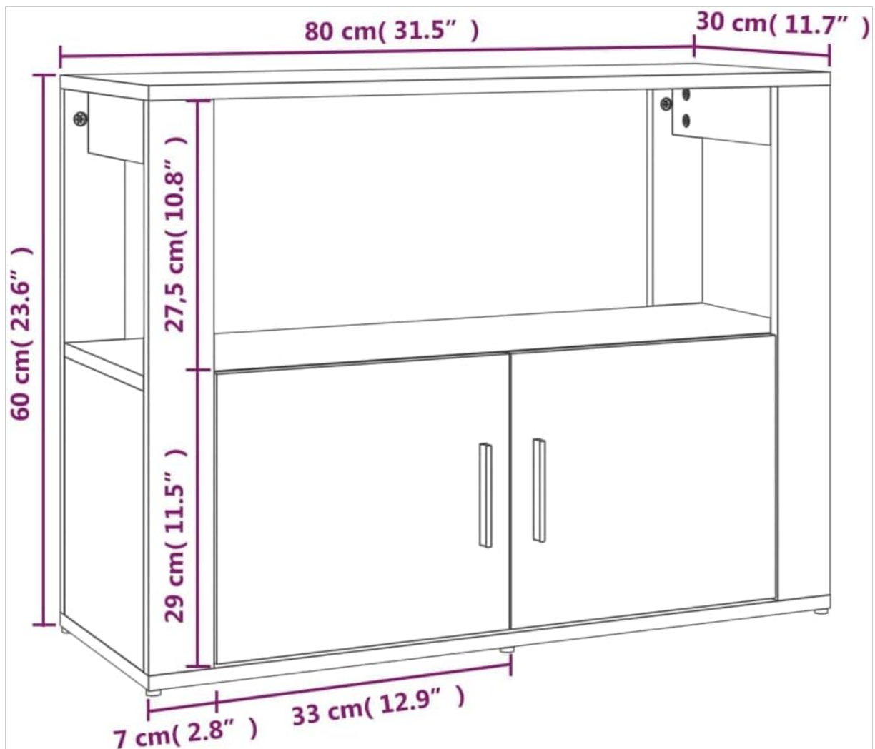
Image 2: Technical drawing showing the dimensions of the cabinet. The overall dimensions are 80 cm (31.5") wide, 30 cm (11.7") deep, and 60 cm (23.6") high. The internal shelf height is 27.5 cm (10.8") and the lower compartment height is 29 cm (11.5").
