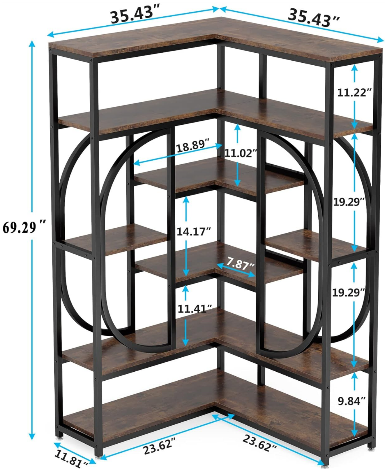
Figure 3.1: Product dimensions, useful for identifying components during assembly.
