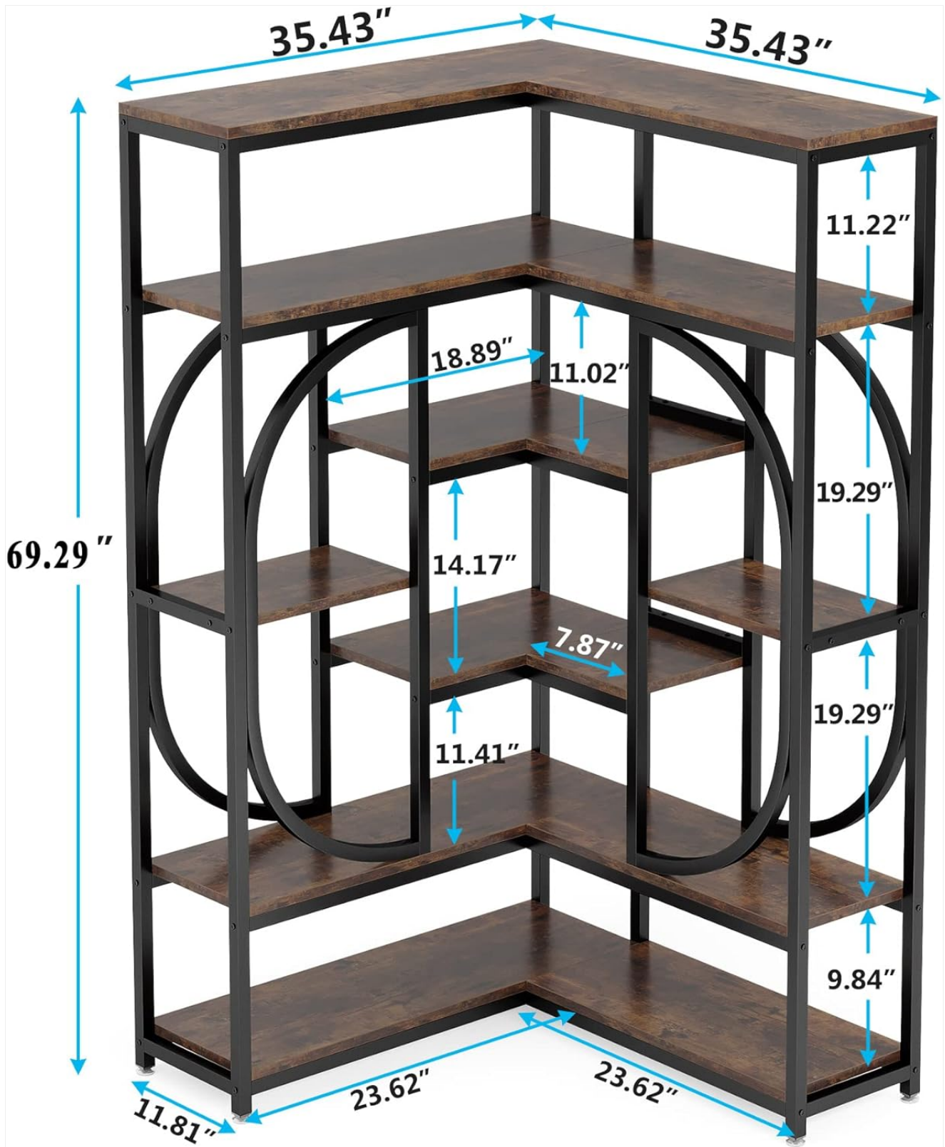
Figure 8.1: Detailed dimensions of the bookshelf.
