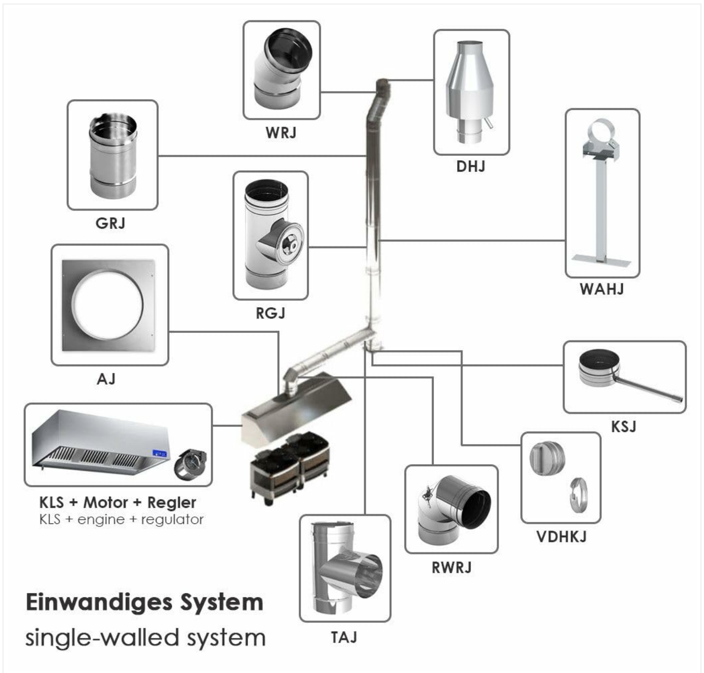
Figure 2: Overview of a single-walled exhaust system, illustrating various components for installation.
