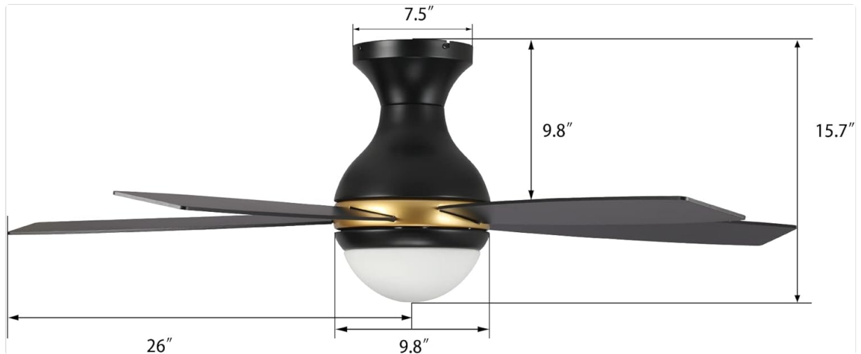
Image 4.1: Diagram illustrating the dimensions of the Carro Twister 52-Inch Ceiling Fan, including blade span, downrod length, and overall height.
